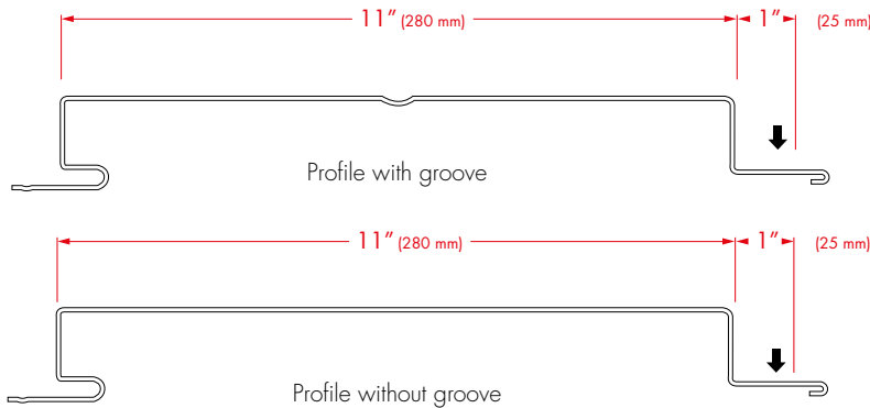
With groove
